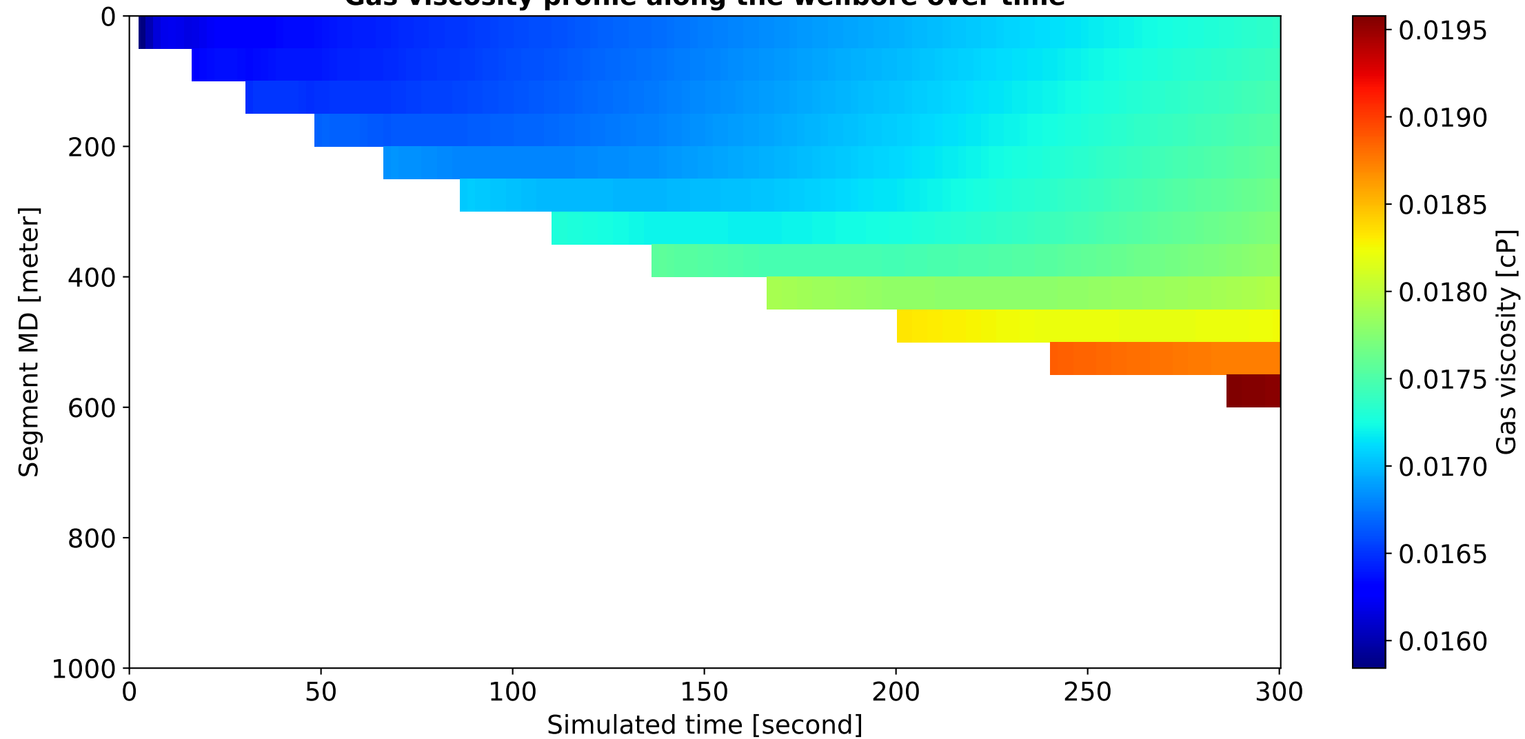
Gas viscosity profile along the wellbore over time
